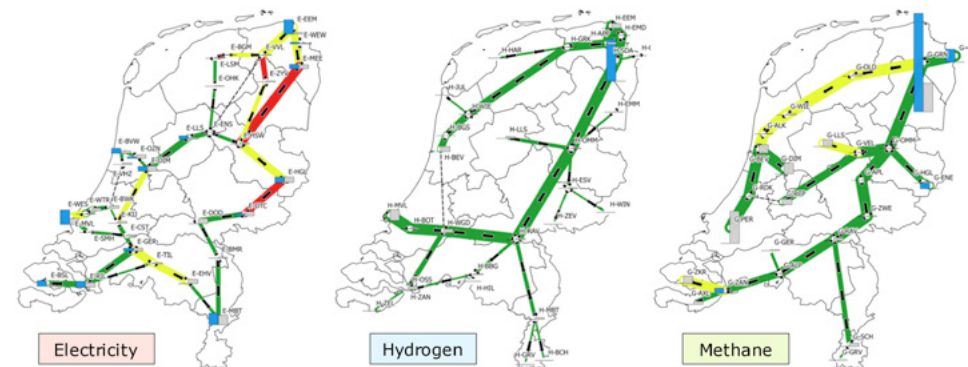
Figure 7: Intensity representation of a flow pattern for a typical snapshot (green = moderate loading; yellow = high loading; red = overloaded; line width proportional to flow)
