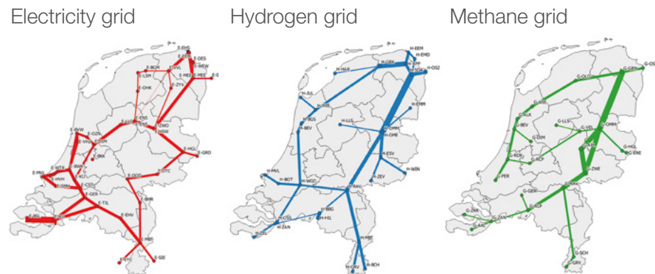
Figure 2: Geographic overview of assumed topologies for the Dutch gas and electricity infrastructures. (Line thickness represents maximum available transport capacity. Visual representation of gas and electricity capacities is not proportional.)
