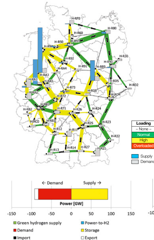
Figure 17: Snapshot of a ‘Dunkelflaute’ situation at the end of January at 6 p.m. (Local, hour 474) in Germany.
