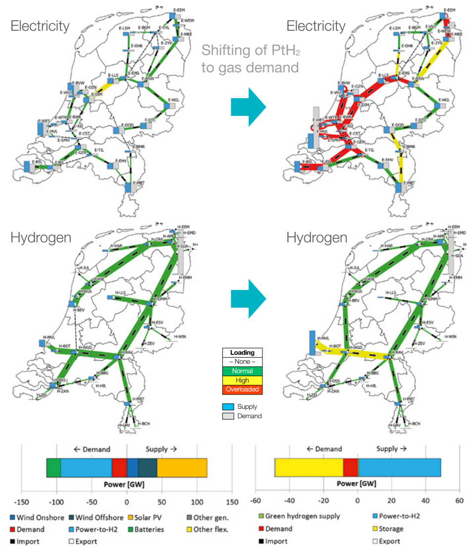
Figure 9: Impact of electrolyser location on electricity flows in the Netherlands. Snapshot 4044 (high demand and high infeed of renewable energy), with electrolyzers located close to renewable electricity supply (left) and close to hydrogen demand (right).
