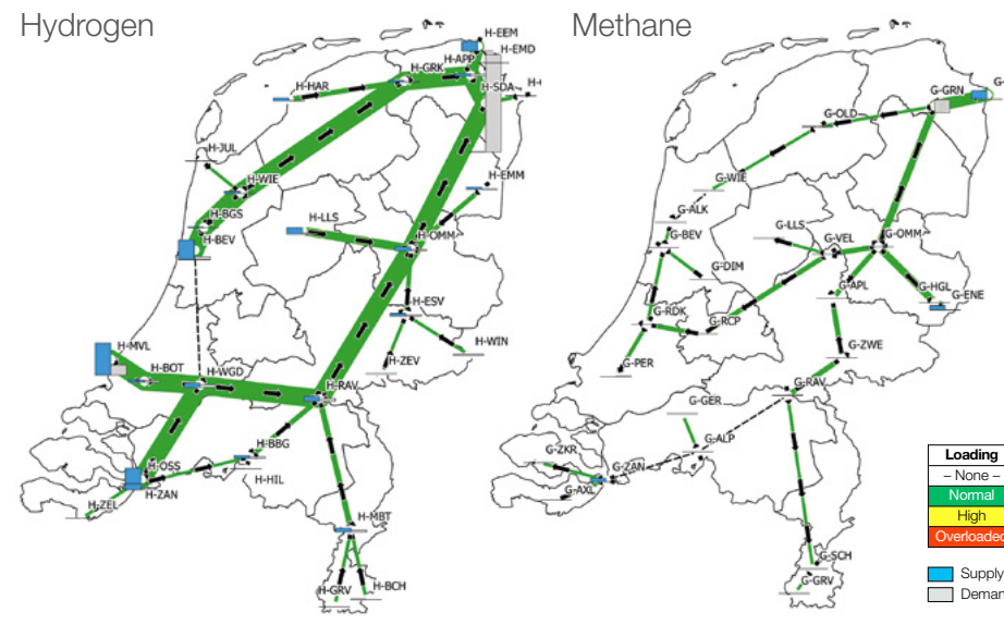
Figure 14: Results of model run for situation with low demand and extensive P2G conversion (National, hour 4044) in the Netherlands.
