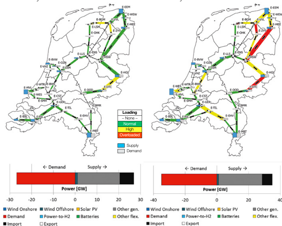
Figure 11: Model results for Dutch snapshots with high demand (Left: National, hour 7746 / Right: Local, hour 954).
