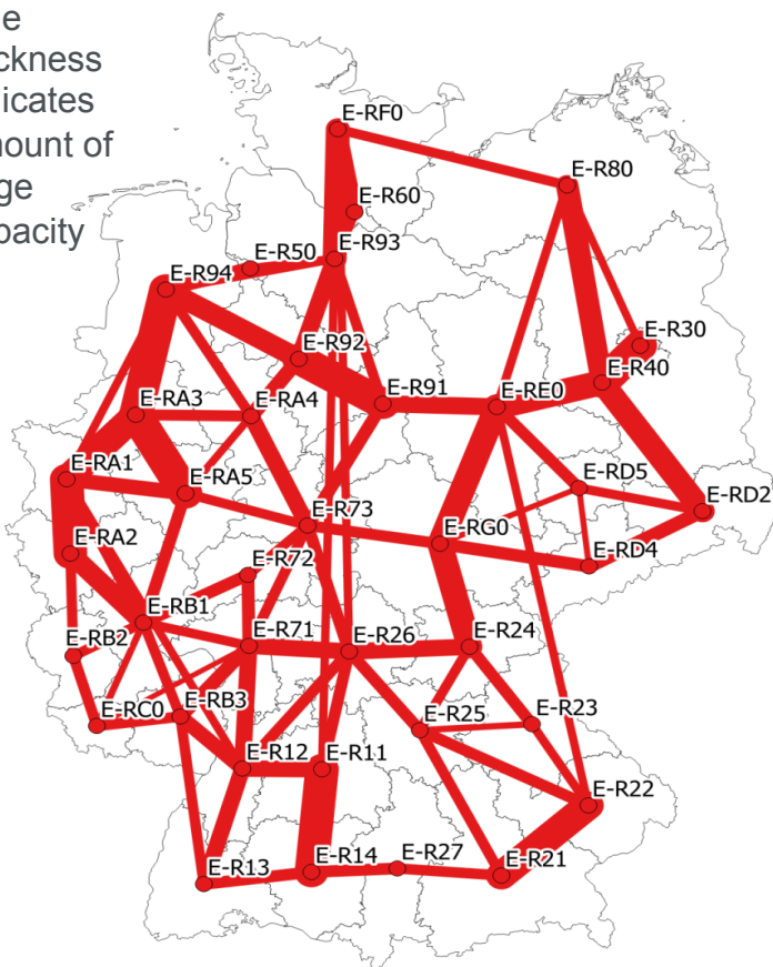
Line capacities (2030)
