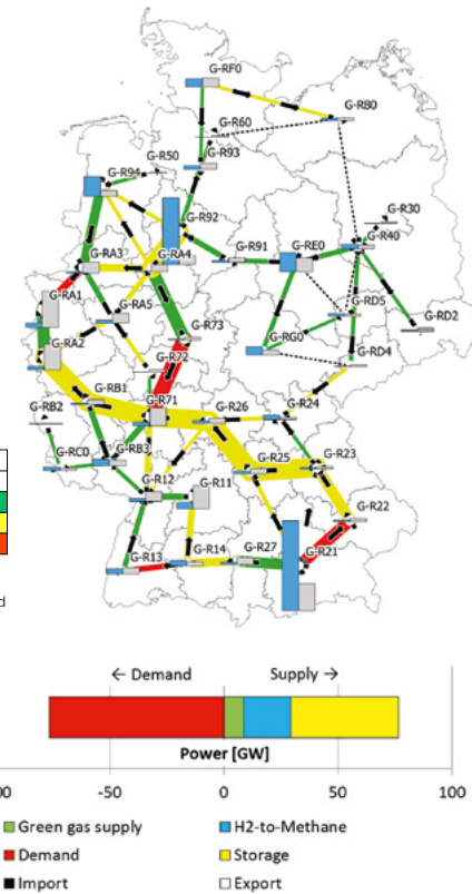
Figure 17: Snapshot of a ‘Dunkelflaute’ situation at the end of January at 6 p.m. (Local, hour 474) in Germany.
