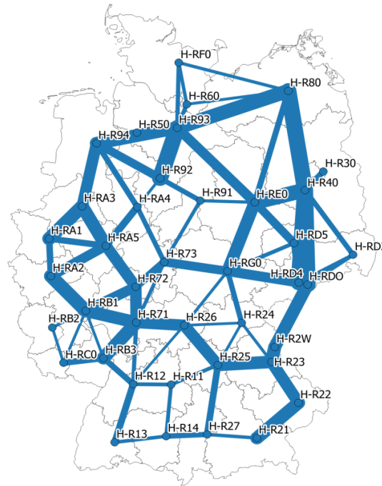
Hydrogen grid
