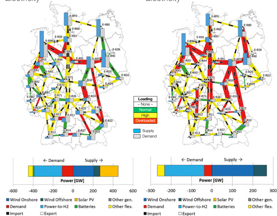
Electricity
